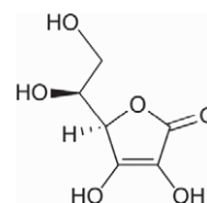
Fig. 2. Chemical structure of ascorbic acid (AA)
